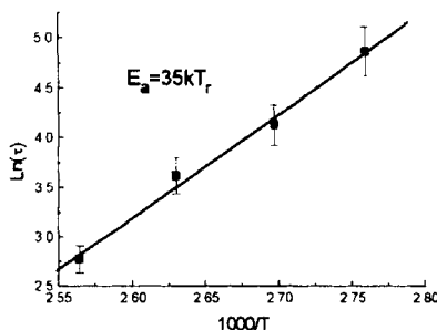
FIGURE 5 The dependence of anisotropy erasure time on the temperature of an isotropic phase of the polymer film.
