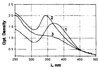
FIGURE 2 Absorption spectra of (1) non-irradiated film and irradiated by non-polarized light: linearly polarized testing beam is (2) in plane of incidence and (3) perpendicular to it. For (2) and (3) angle of testing beam incidence is 45^\circ .
