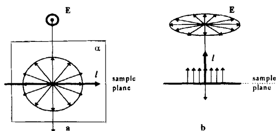
FIGURE 3 Angle distribution of azobenzene fragments under irradiation with polarized (a) and non-polarized light (b).
