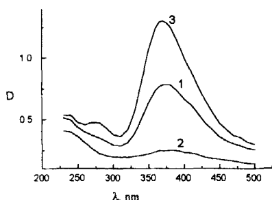
FIGURE 1 Absorption spectra of the azo-polymer film: 1 - non-irradiated; 2, 3 - after irradiation with polarized light, polarization of the testing beam is parallel (2) or perpendicular (3) to polarization of the irradiating beam.
